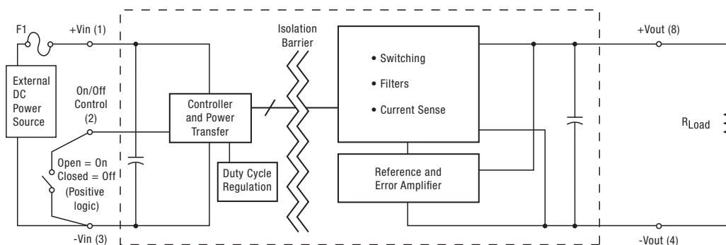
Figure 1. Connection Diagram Typical topology is shown. Murata Power Solutions recommends an external fuse at F1.
